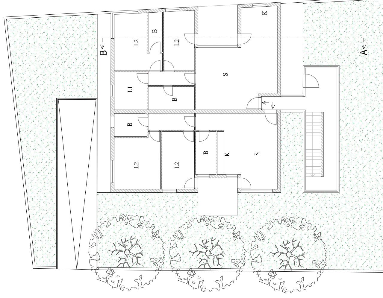
Piano Terra
