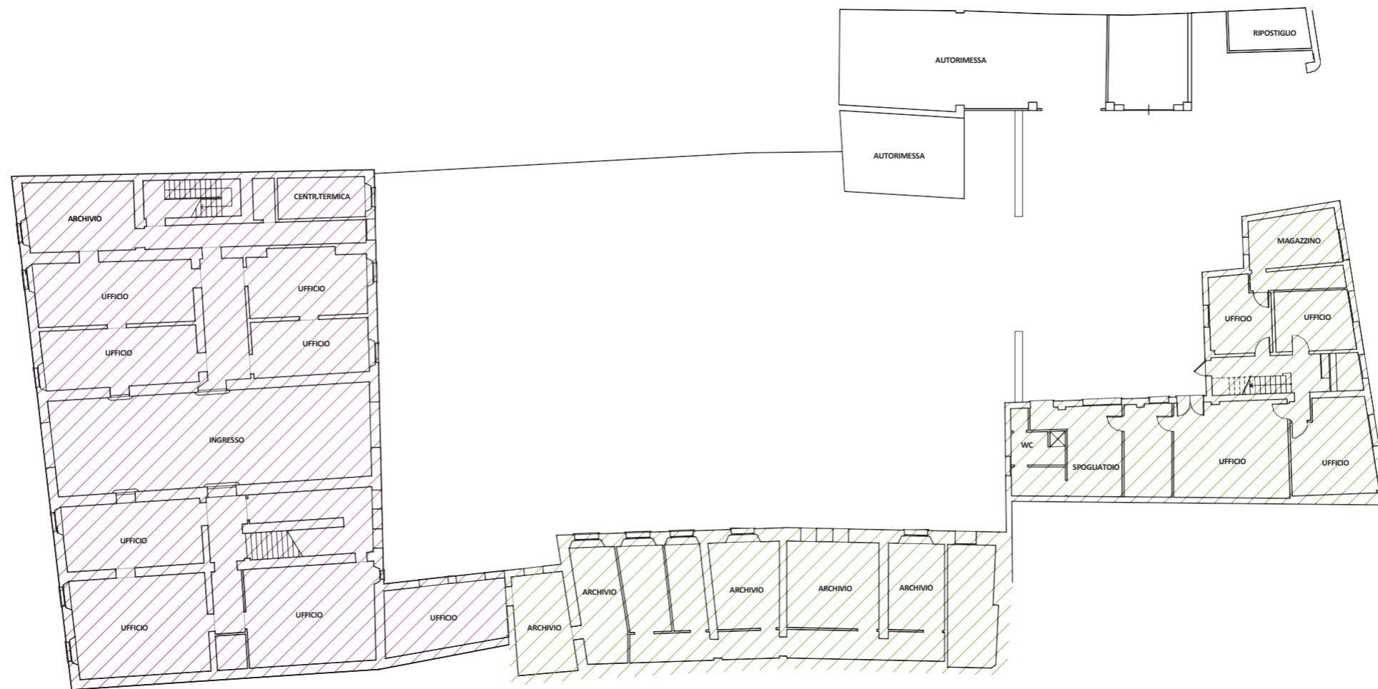
PIANO TERRA
